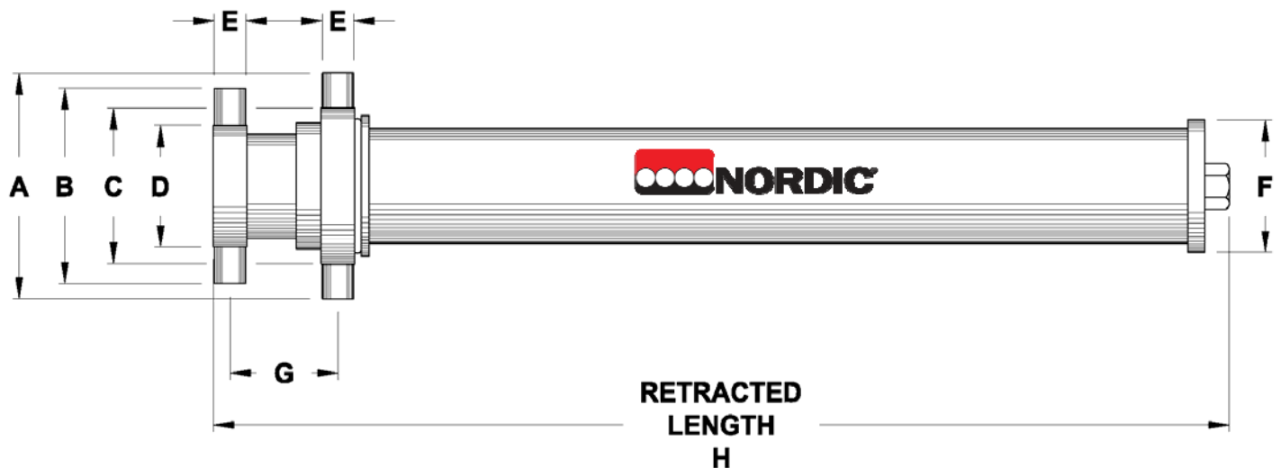
Telescopic Cylinder With Optional Saddle And Box Mounting Pivot Blocks
